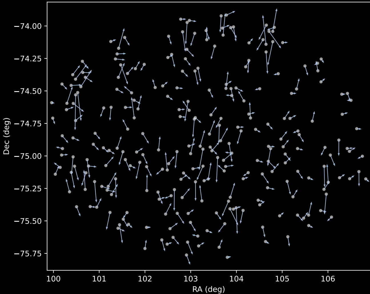
GALAH DR4 Cluster 1 Proper Motion Vectors (n=259)
