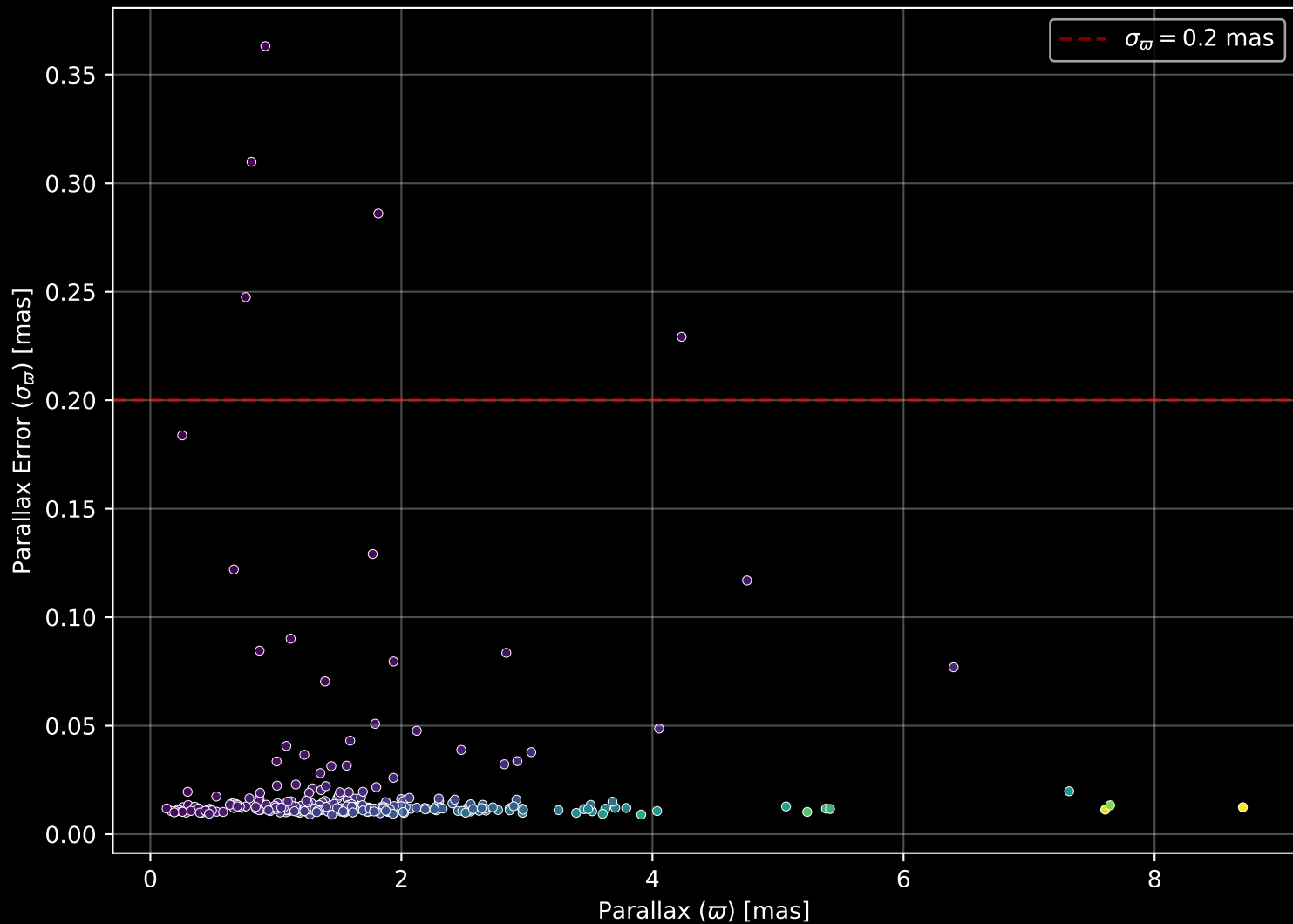
GALAH DR4 Field: [133] Parallax Quality (n= 296)
