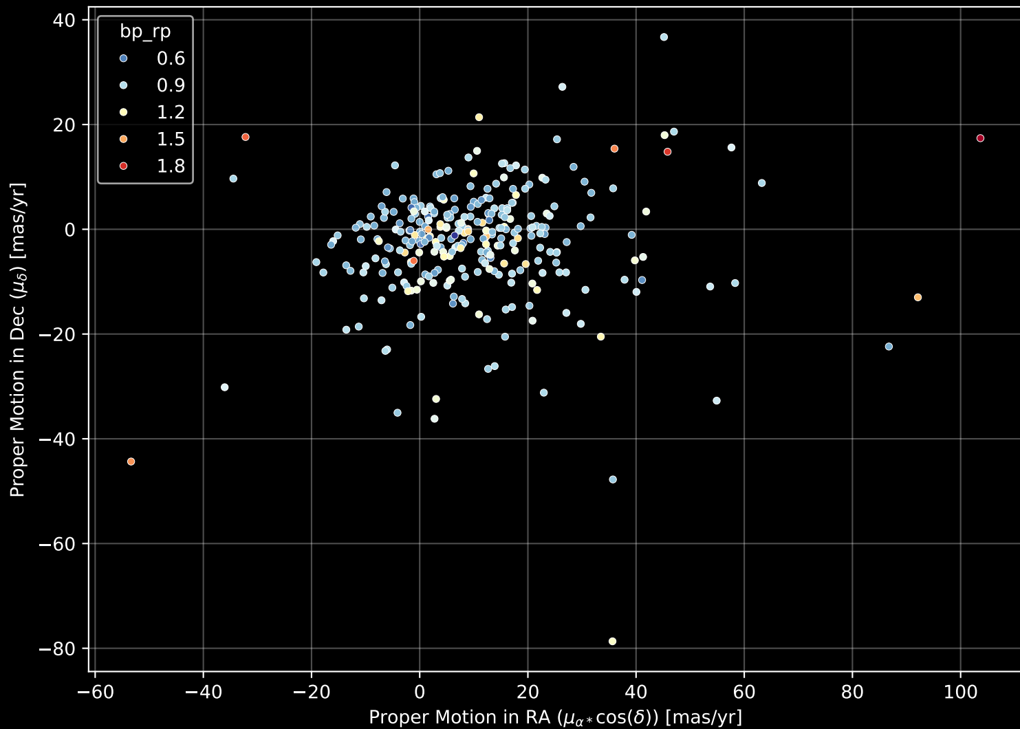
GALAH DR4 Field: [133] Proper Motion Diagram (n= 296)
